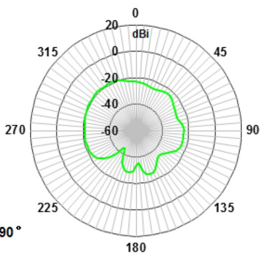
Vertical Polarization
